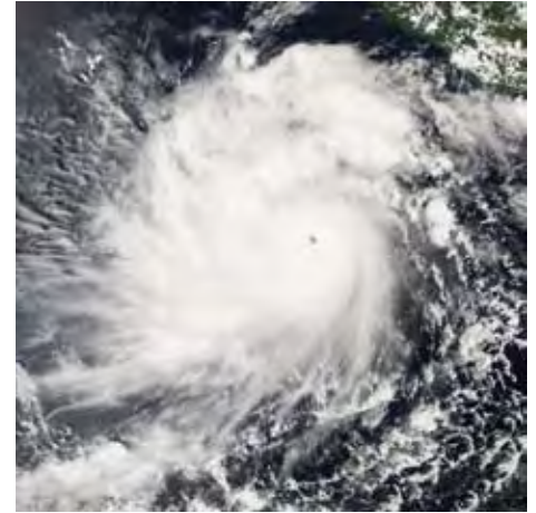
Figure 5. Satellite image of hurricane Javier on September 13, 2004 approximately 610 miles southeast of Cabo San Lucas, Mexico. Source: Jesse Allen, NASA Earth Observatory, data from the MODIS Rapid Response team
