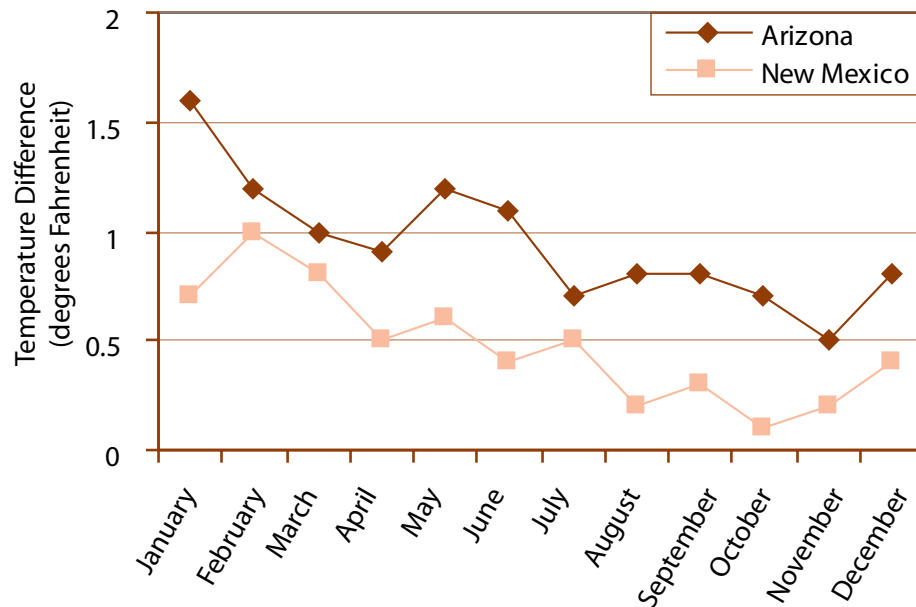
Figure 2. The difference between Arizona and New Mexico's average monthly temperatures in the past five years (2000–2005) compared to the full record (1895–2005) is shown above. The difference was most pronounced in winter and spring. Data: Western Regional Climate Center.
