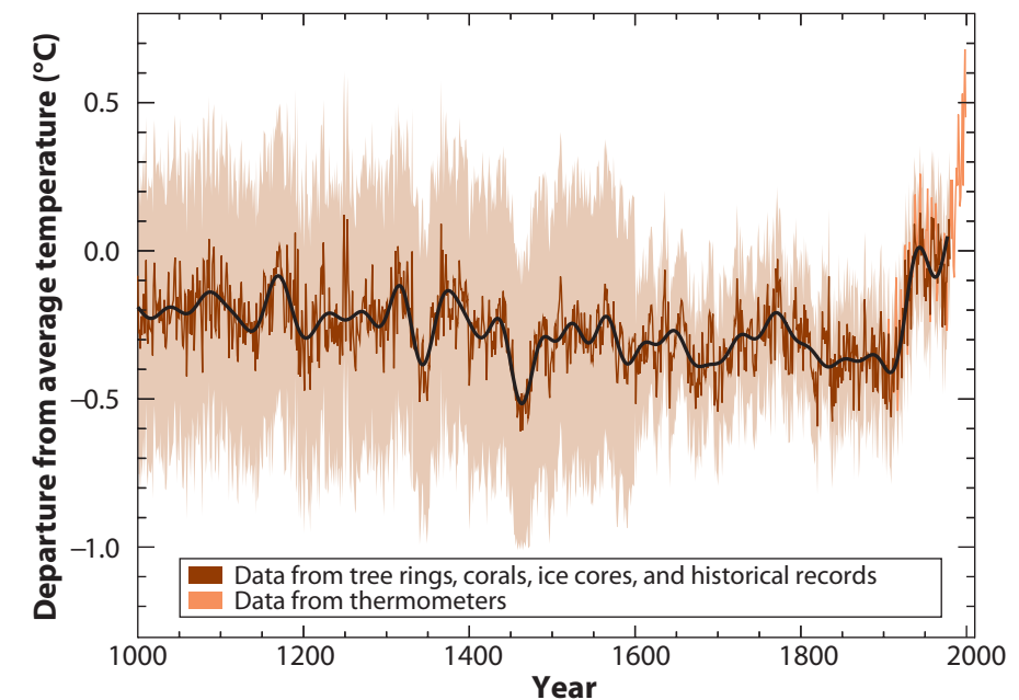
Figure 2. The instrumental record of northern hemisphere temperature (pink) is superimposed on a 1,000-year temperature record for northern hemisphere reconstructed from annual tree rings, coral growth, and ice core layers (brown, with range of potential error shown in tan and "smoothed" average shown in black). Its shape, with an abrupt rise in modern times, has led some to dub the record a "hockey stick." Source: Intergovernmental Panel on Climate Change Third Annual Assessment, 2001.
