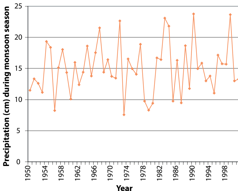
Figure 2. Annual precipitation in the monsoon region during the monsoon season fluctuates widely by year, but the fluctuations show no ongoing trend toward an increase in seasonal rainfall in recent years. Graphic based on 1950–2001 dataset accessible from Andrew Ellis’ website at http://geography.asu.edu/azclimate/monsdat.htm .
