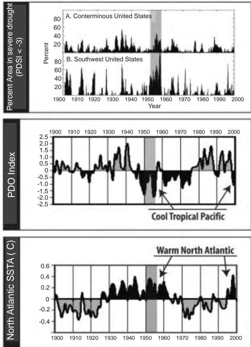
Figure 1. Opposing shifts in tropical Pacific and North Atlantic Ocean temperatures may foretell persistence of disastrous, multiyear droughts across the North American continent. During most of the 1950s, drought conditions characterized the Southwest (top), which in this analysis includes Arizona, New Mexico, Utah, Colorado and parts of Texas and Oklahoma. The gray shading shows the same time frame in all figures, including those of two indices that appear linked to long-term drought in the Southwest, the PDO (middle) and AMO (bottom). The indices returned to their 1950s pattern in 1999, which some see as an ominous sign that long-term drought may be in store. All figures provided by Julio Betancourt.
