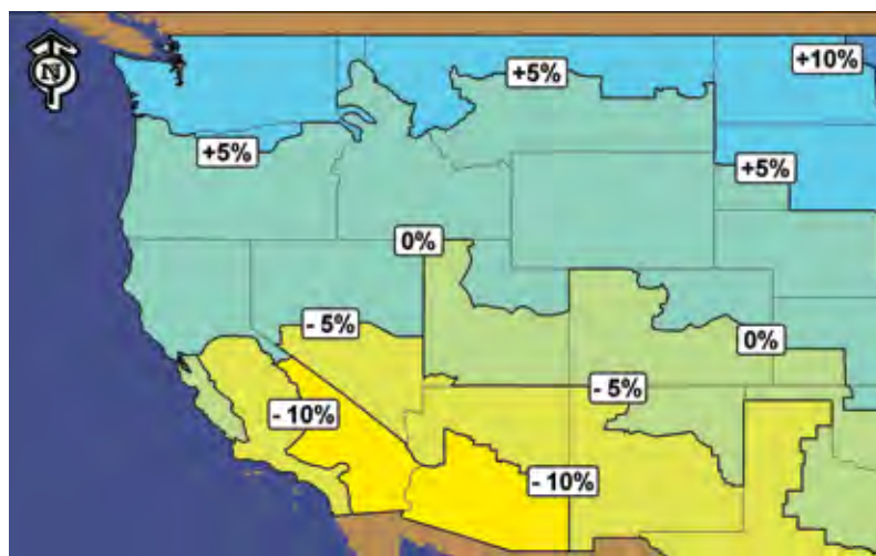
Figure 3. Projected annual precipitation changes from 2091 to 2100.*
