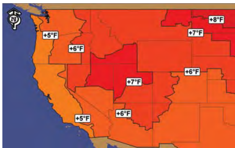
Figure 2. Projected December–February temperature changes from 2091 to 2100.*
