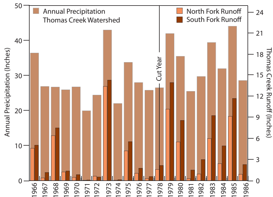
Figure 1. The South Fork of Thomas Creek in the White Mountains had a slight tendency to produce more “runoff,” or water yield from overland flow, before a logging treatment that was completed on the South Fork of the watershed in 1978. After the treatment, this tendency was more pronounced, as the above graphic illustrates. However, the main difference occurred in years of high precipitation. On the graphic, the scale for precipitation for the Thomas Creek watershed is on the left, while the scale for runoff values is given on the right. Data from 1989 University of Arizona dissertation of Gerald Gottfried, School of Natural Resources.
