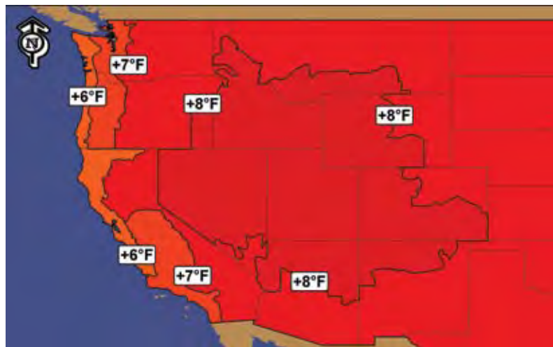
Figure 1. Projected June–August temperature changes from 2091 to 2100.*
