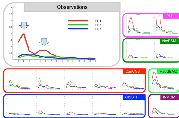
Fig. 3 Power spectra of the first three principal components of North Atlantic SSTs for observations and historical simulations. The abscissa denotes number of cycles per 140 years. Blue arrows indicate the observed spectral peaks at \sim 70 and \sim 25 years.
