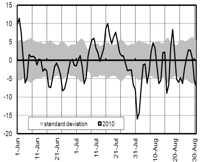
Fig. 5.7 Time series of average sea level pressure anomaly (unit: hPa) over the Sea of Okhotsk ( 45^{\circ}\text{N} - 60^{\circ}\text{N} , 140^{\circ}\text{E} - 155^{\circ}\text{E} ) from June to August 2010. The thick line indicates daily mean values of the area-averaged sea level pressure anomaly over the region. The gray shading denotes the range of one standard deviation.
