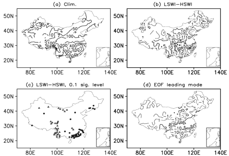
Fig. 2 (a) Climatology of the springtime accumulated precipitation (mm) during 1979–2004, (b) composite difference between the LSWI and HSWI cases, (c) distribution of stations for which the composite difference exceeds the 0.1 level of significance [triangles (dots) indicate significant positive (negative) difference], and (d) the spatial pattern of springtime rainfall anomalies of the leading EOF mode for the period 1979–2004.
