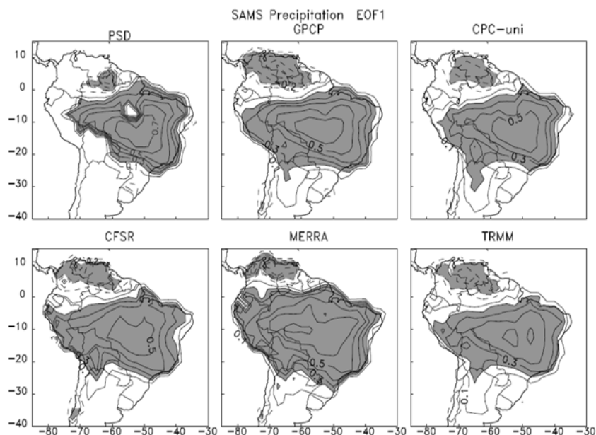
Fig. 1 First EOF patterns described as correlations between the first temporal coefficient (PC1) and precipitation anomalies. Solid (dashed) contours indicate positive (negative) correlations at 0.1 intervals (zero contours omitted). Shadings indicate correlations \geq 0.2 ( \leq -0.2 ) and are significant at 5%. Data grid spacing: 2.5^\circ lat/lon.
