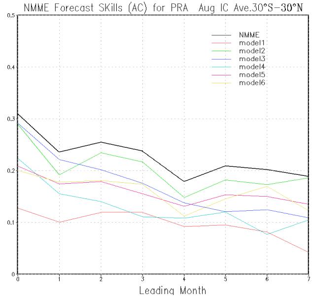
Fig. 5a NMME forecast skills (black line) and individual models (color lines) for precipitation averaged 30S-30N with August ICs.
