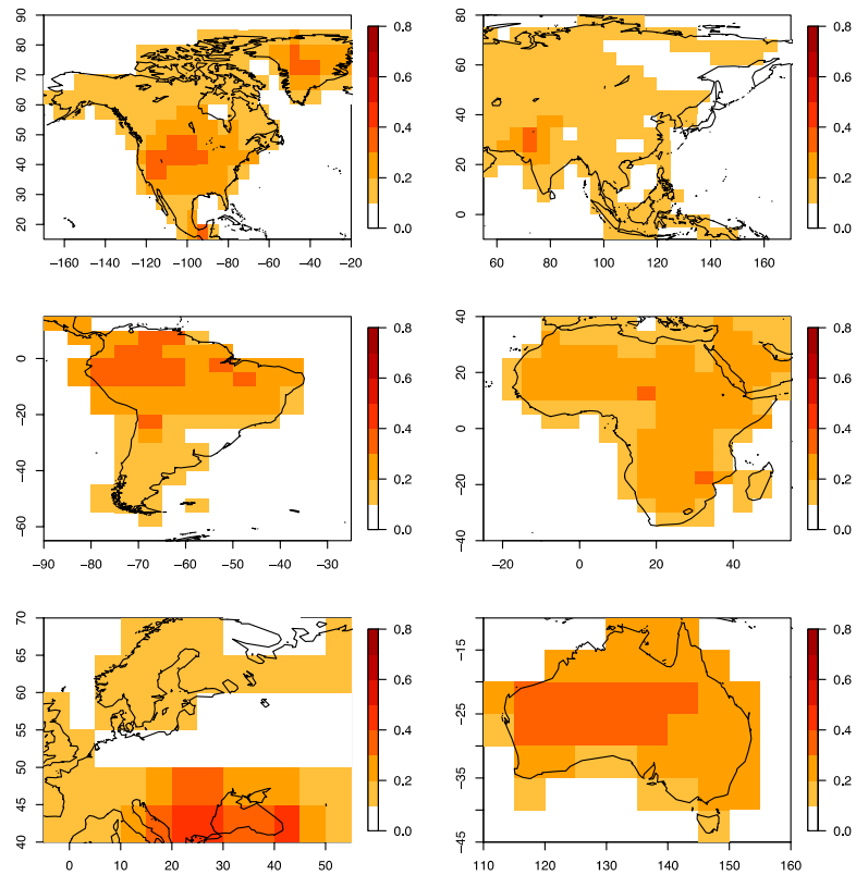
Fig. 4 Spatial pattern of the leading component of JAS mean surface air temperature in verification data. The spatial pattern has units of degree Kelvin and indicates deviations from the time mean.
