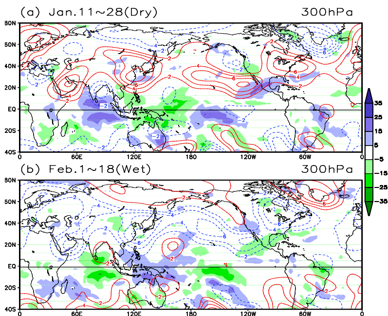
Fig. 4 Intraseasonal anomalies of OLR and 300hPa streamfunction on the days when convection over the tropical central Pacific in (a) dry and (b) wet phases. The OLR is shaded. The 300hPa streamfunction is drawn in contour.
