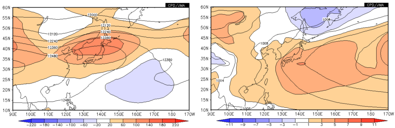
Fig. 5.5 Monthly-mean atmospheric circulation around Japan for August 2010. Left panel: The contours indicate 200-hPa height at intervals of 120 m. Right panel: The contours indicate sea level pressure at intervals of 4 hPa. The shading shows their anomalies.
