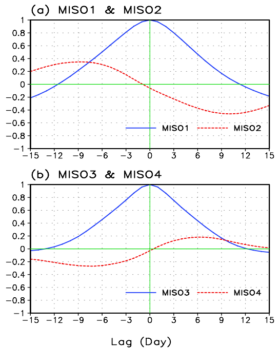
Fig. 3 Lead-lag correlations (a) between the MISO 1 and itself, and with MISO 2 and (b) between the MISO 3 and itself, and with MISO 4 during MJJAS.
