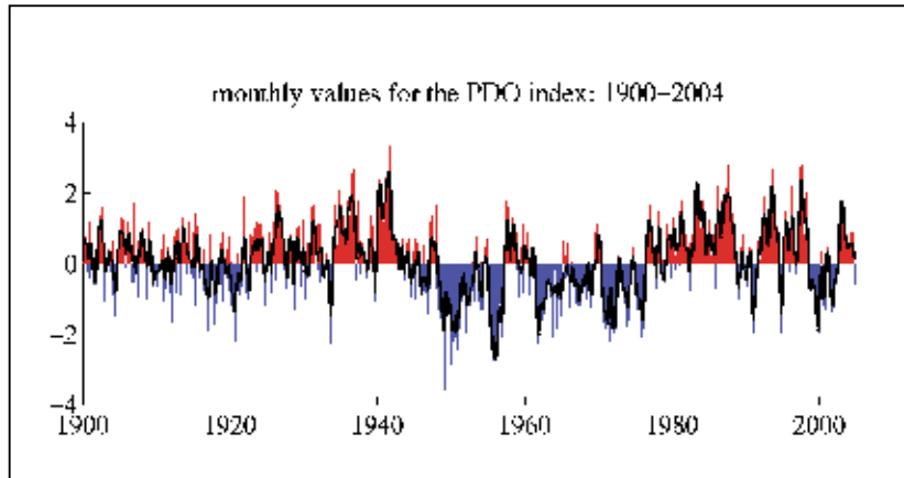
Figure 5. Pacific Decadal Oscillation (PDO) monthly index, 1900-2004. Red shading indicates warm phase, and blue indicates cool phase. Credit: http://tao.atmos.washington.edu/pdo/ .
