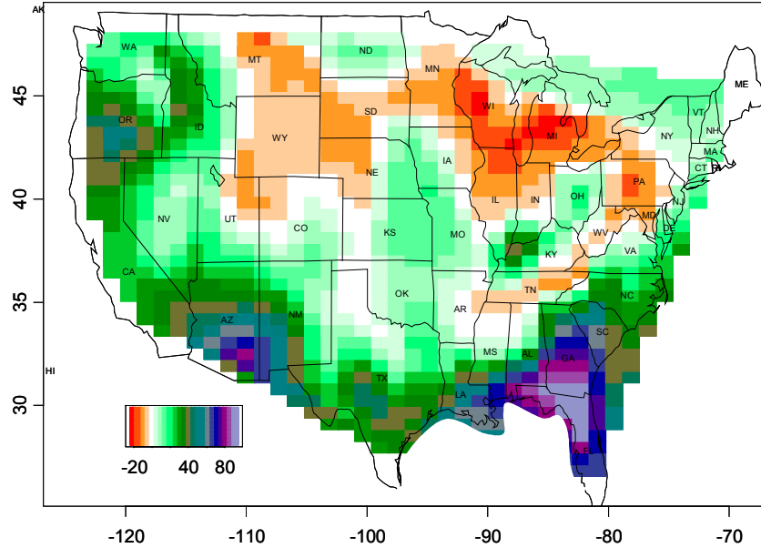
Figure 5: Skill scores for December to April precipitation during El Niño and La Niña events, predicted at 0.5 to 6.5 months in advance. Note the strong skill in the Southwest, Southeast, and Northwest; areas where ENSO most directly affects precipitation. In the Colorado River Basin strong positive skill is confined to the lower basin, not in the Rocky Mountains which provide about 90% of the runoff. Note the negative skill in NE Utah and SW Wyoming, the headwater areas of the Green River. Precipitation skill from CPC forecasts during non-ENSO years in all seasons is negligible in the entire country (not shown.)
