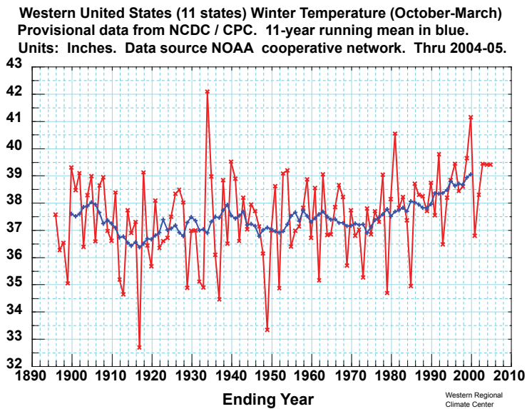
Figure 6. Western U.S. winter precipitation and temperature, 1895-2005.
